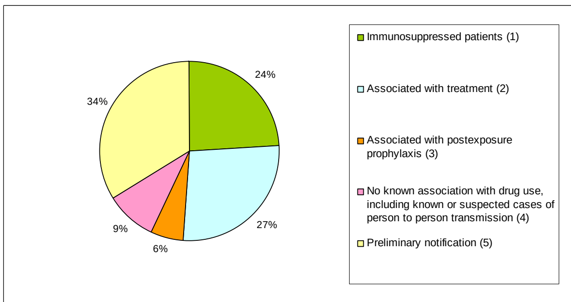
Figure 1: Proportion of the clinical background of reported cases of oseltamivir resistance (as of 23 June 2010). Cases are classified first by identifying those that occur in severely immunocompromised patients (1). The remaining cases are then classified as either occurring during or after oseltamivir treatment (2), associated with post-exposure prophylaxis (3), or occurring in patients who had not used antiviral drugs prior to occurrence of the resistant virus (4). The balance of cases (5) are those where insufficient clinical information is available.
