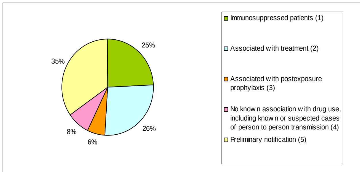
Figure 1: Proportion of the clinical background of reported cases of oseltamivir resistance (as of 14 April 2010). Cases are classified first by identifying those that occur in severely immunocompromised patients (1). The remaining cases are then classified as either occurring during or after oseltamivir treatment (2), associated with post-exposure prophylaxis (3), or occurring in patients who had not used antiviral drugs prior to occurrence of the resistant virus (4). The balance of cases (5) are those where insufficient clinical information is available.
